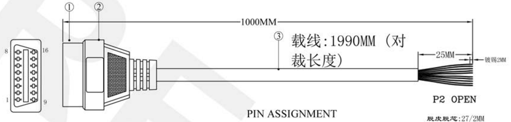
P1 OBDII FEMALE
