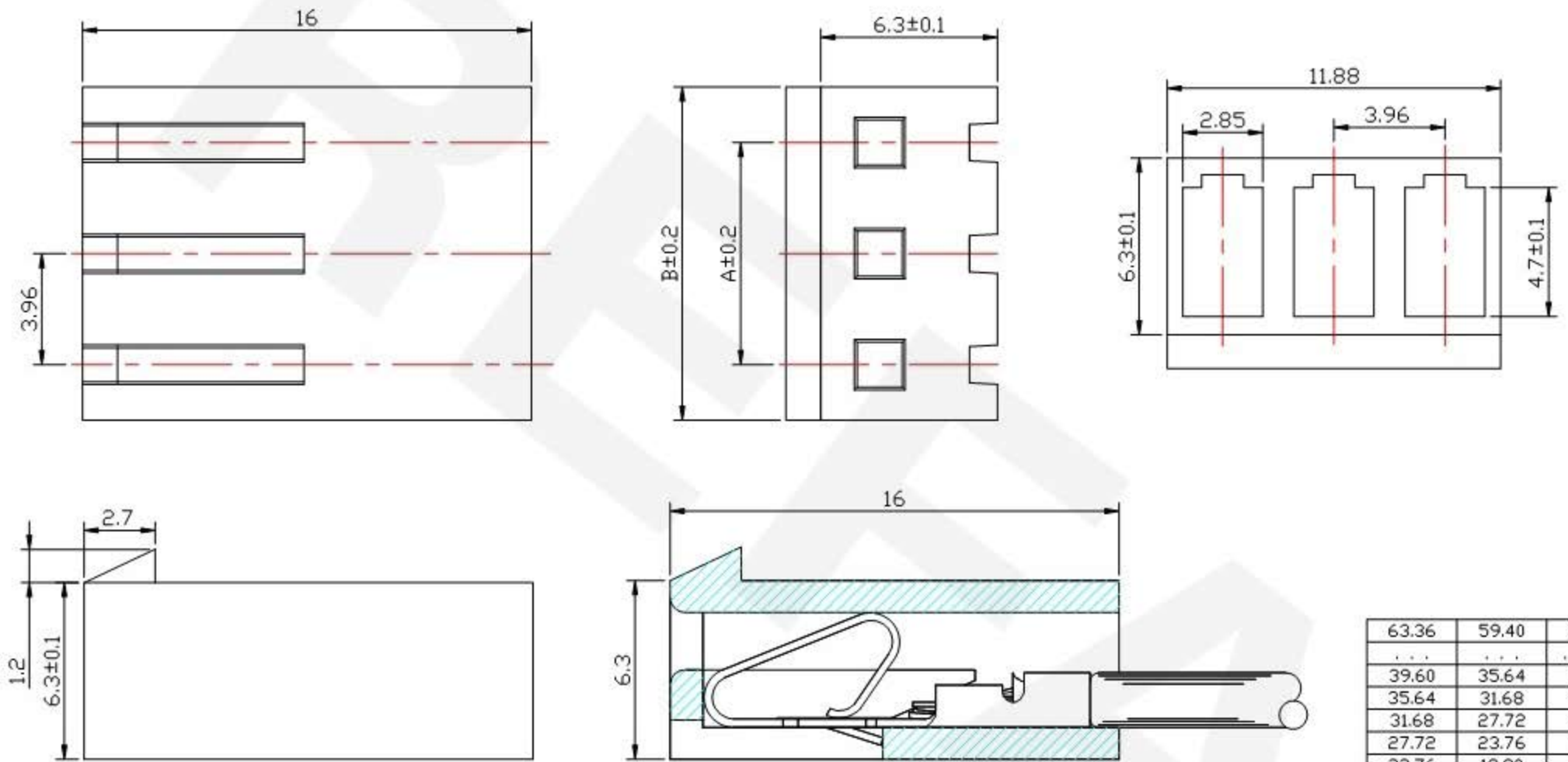
SECTIONAL DRAWING
