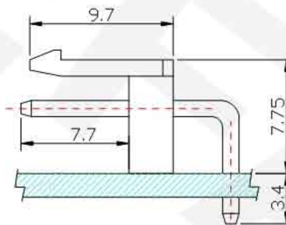
ASSEMBLY LAYOUT
