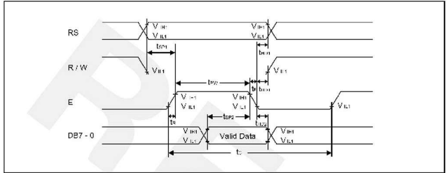
Timing Diagram Writing mode
