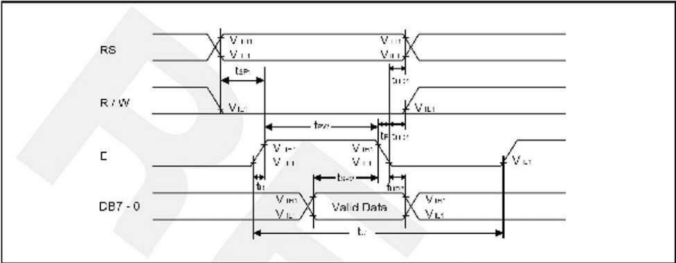
Timing Diagram Writing mode
