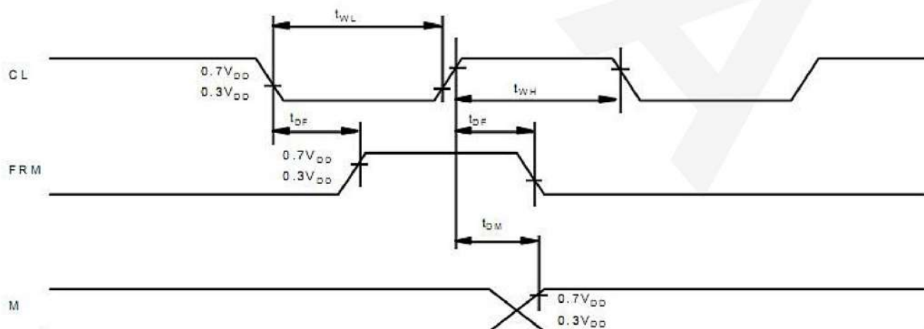
Fig 2. Display control signal waveform
