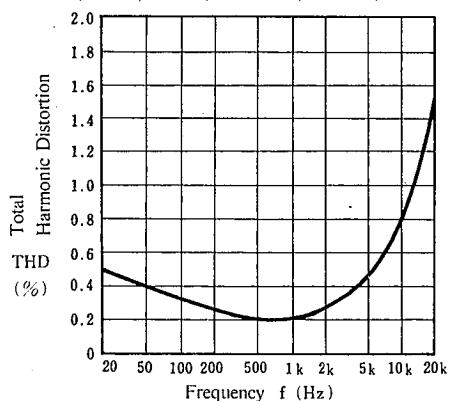
Total Harmonic Distortion vs. Frequency (V + = 6V, R L = 8Ω, P o = 125mW, A v = 26dB, T_a = 25^\circ\text{C} )
