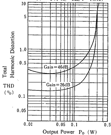
Total Harmonic Distortion vs. Output Power
