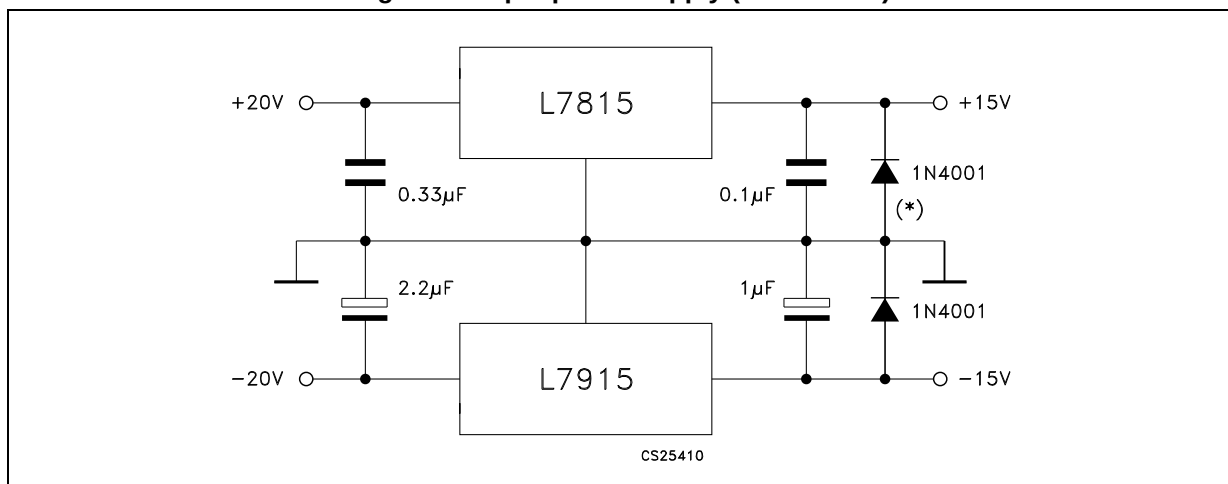
Figure 16. Split power supply ( \pm 15 V - 1 A)
