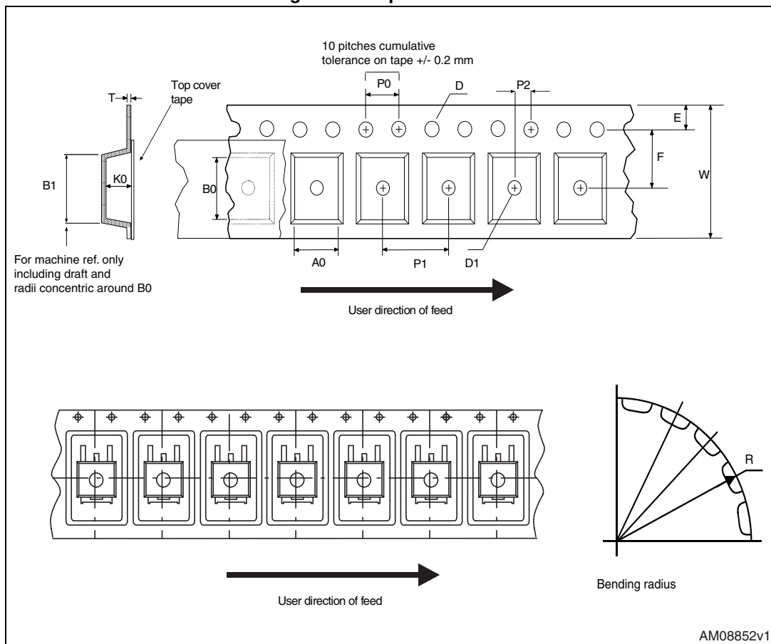
Figure 49. Tape for D 2 PAK
